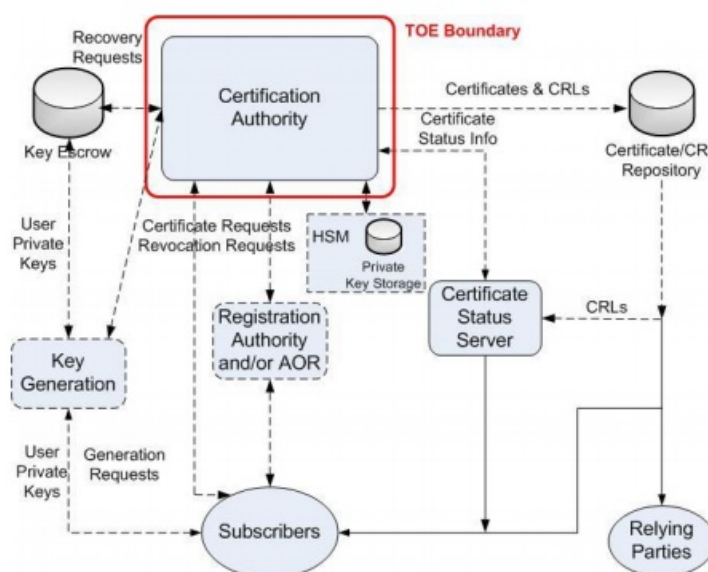
Figure 1: TOE Boundary in Example PKI Architecture
