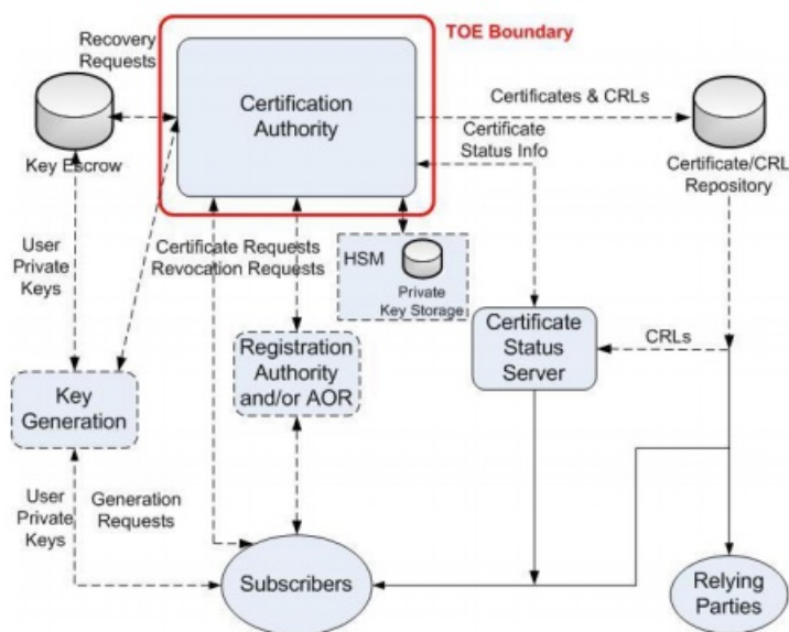
Figure 1: TOE Boundary in Example PKI Architecture
