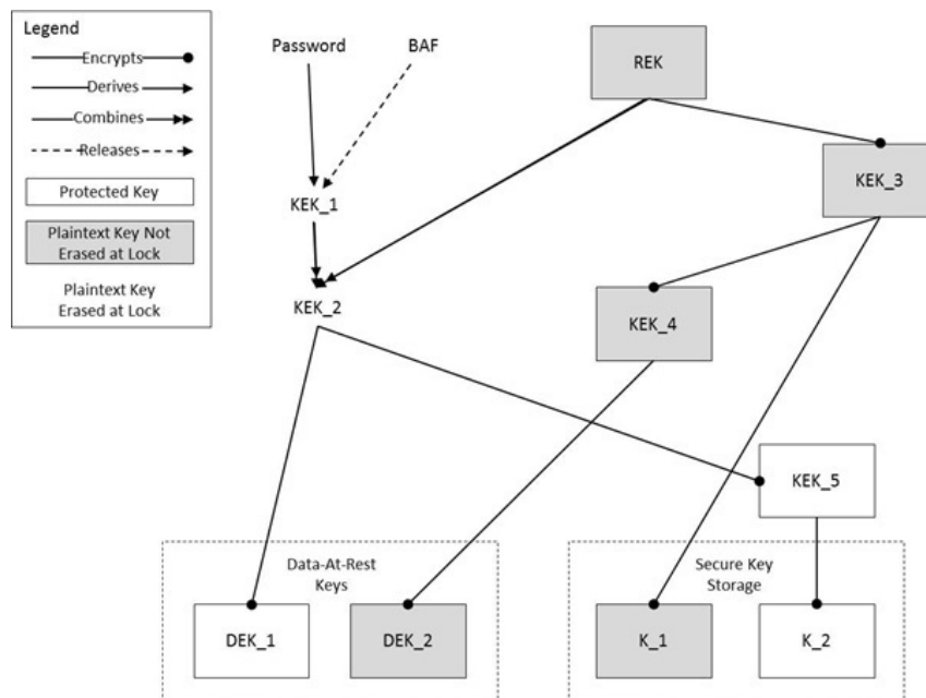
Figure 3: An Illustrative Key Hierarchy
